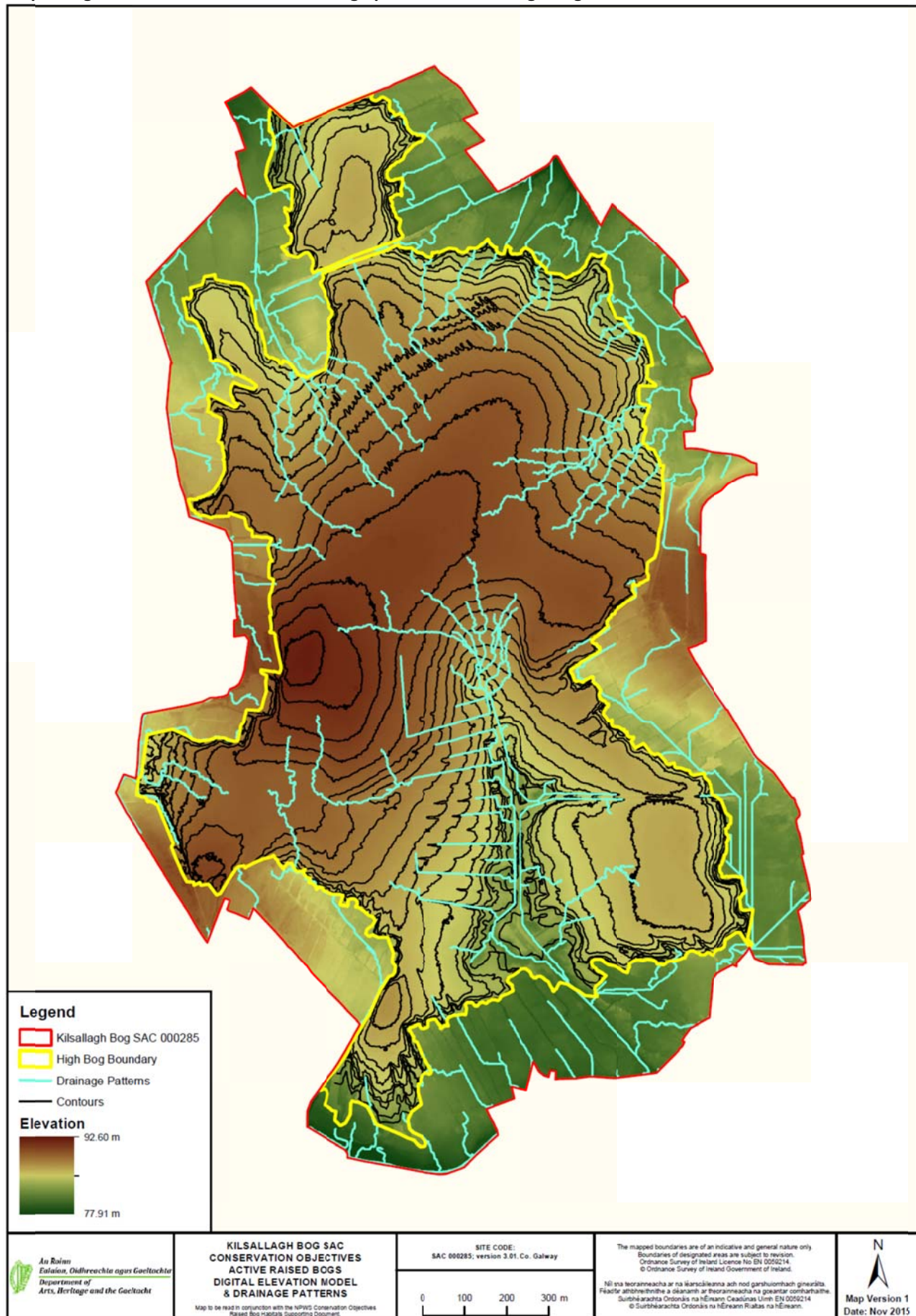
Map 3: Digital elevation model and drainage patterns at Kilsallagh Bog.
