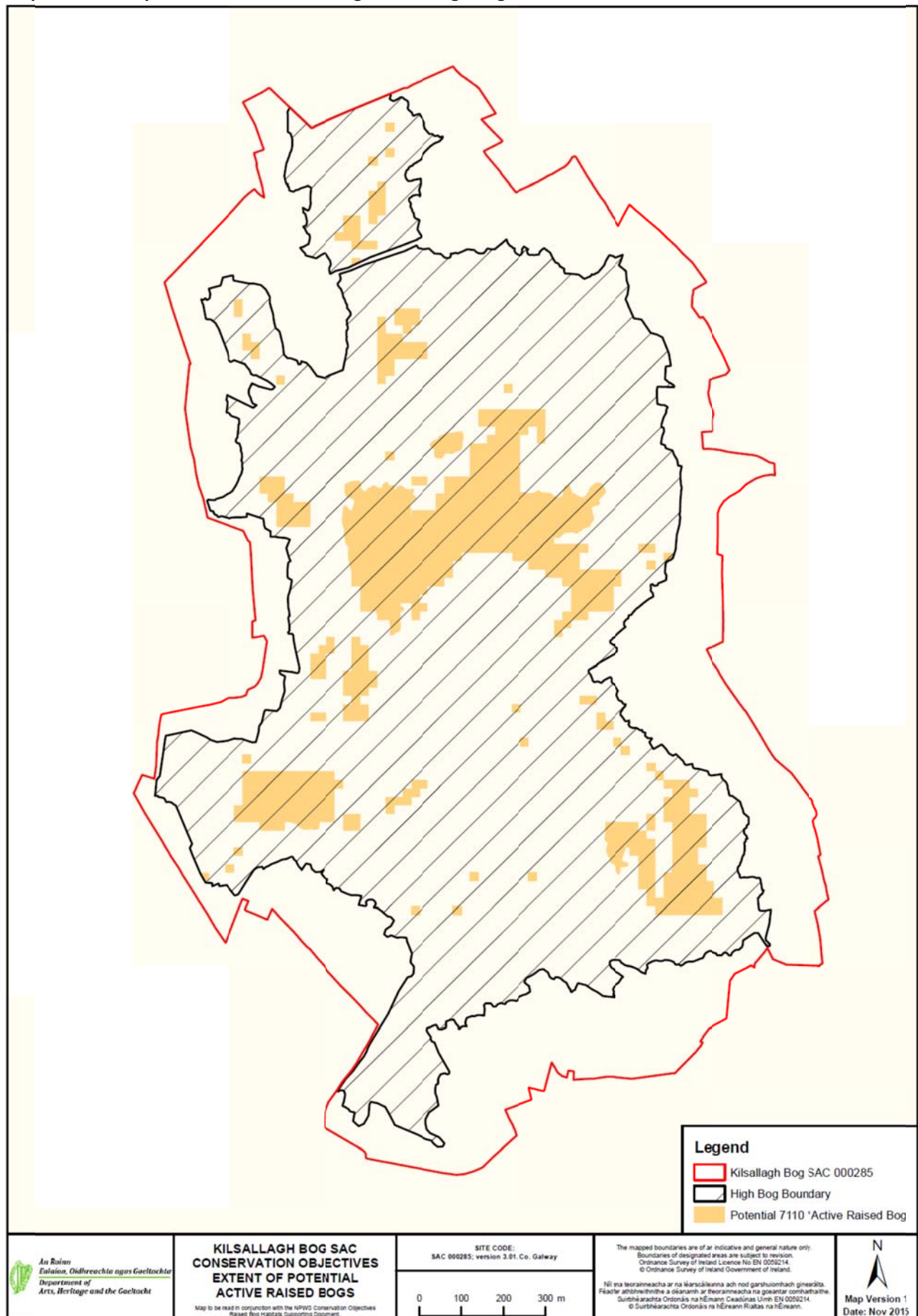
Map 1: Extent of potential active raised bog on Kilsallagh Bog.
