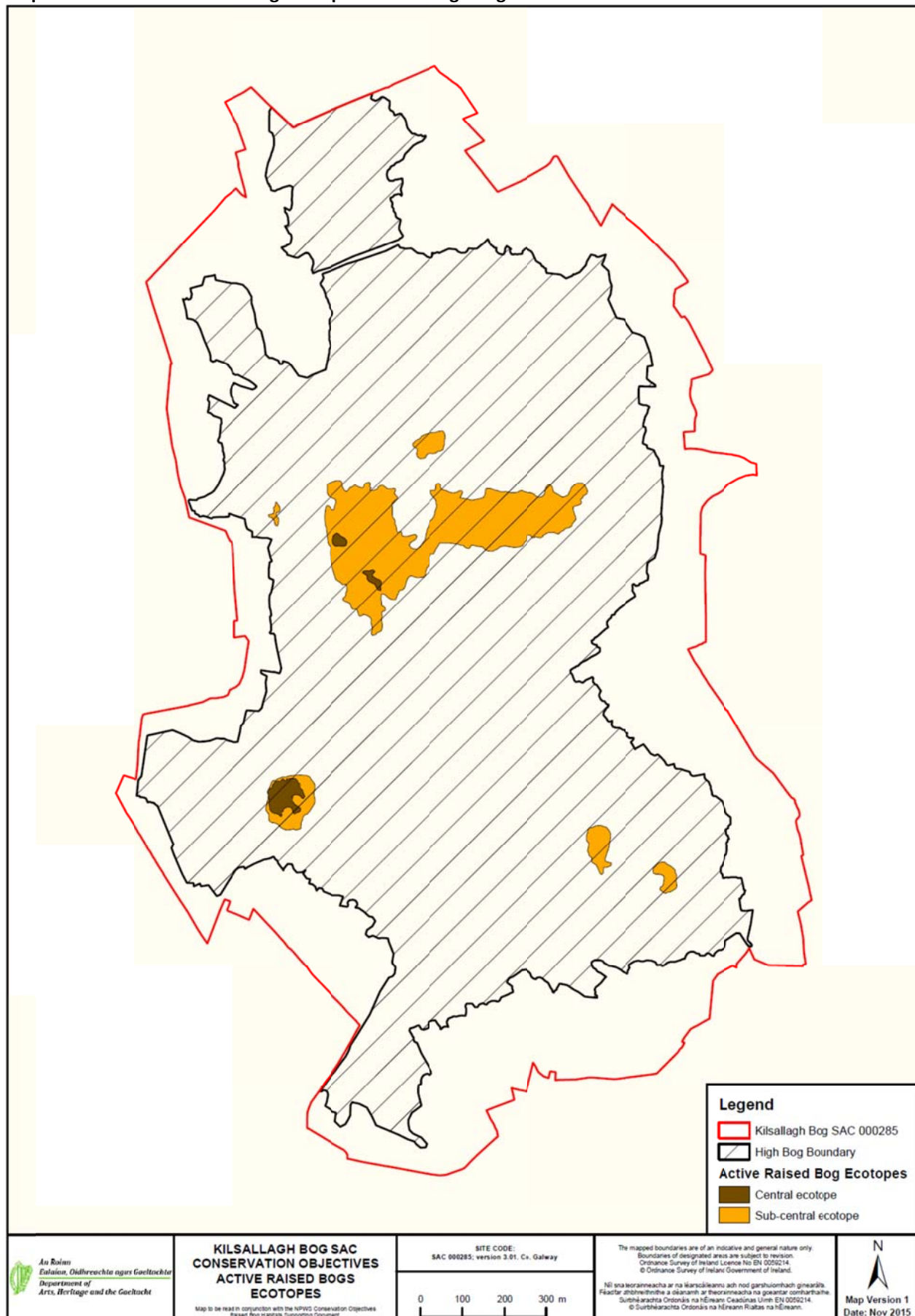
Map 2: Distribution of raised bog ecotopes on Kilsallagh Bog.
